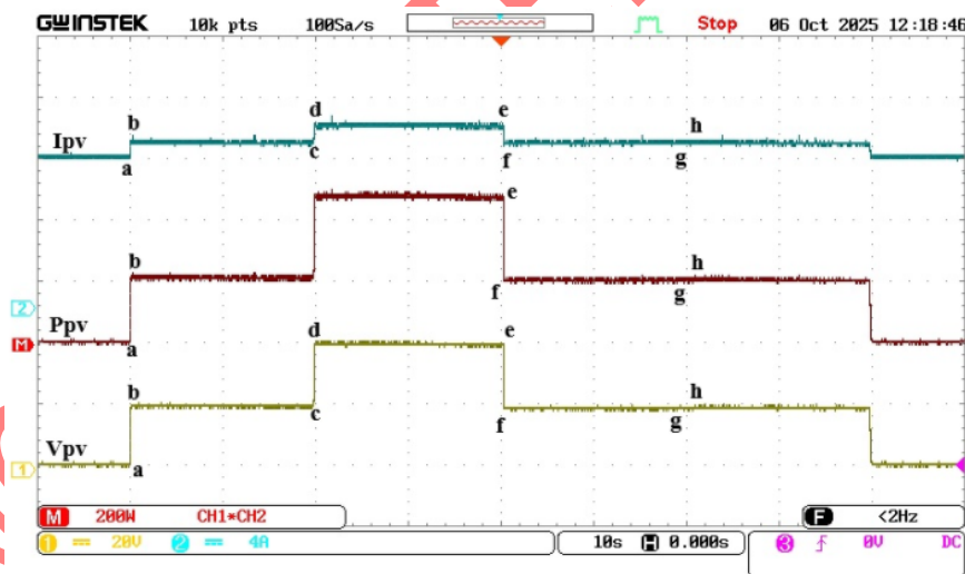
Figure 6. Performance of the OA-P&O MPPT algorithm with the outputs is Vpv, Ppv, and Ipv (scale: 10s/div; Vpv (Ch1) 20V/div; Ipv (Ch2) 4A/div; and Ppv (math trace) 200 W/div)
