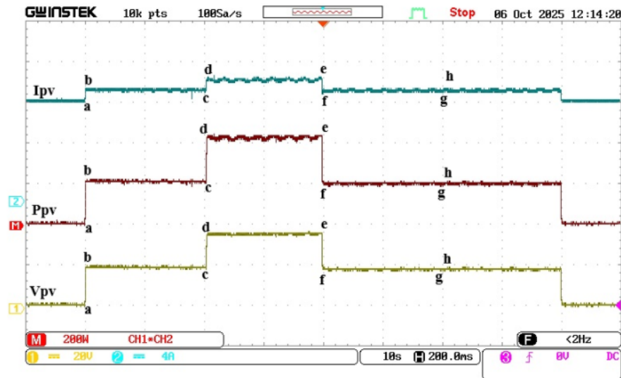
Figure 5. The performance of the conventional P&O MPPT algorithm with the outputs is Vpv, Ppv, and Ipv (scale 10s/div; Vpv (Ch1) 20V/div; Ipv (Ch2) 4A/div; and Ppv (math trace) 200 W/div)
