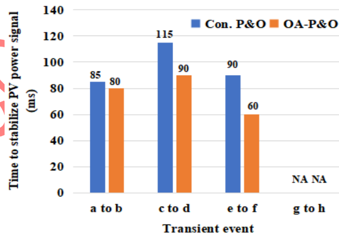
Figure 8. MPPT power stabilization time comparison during transient events
