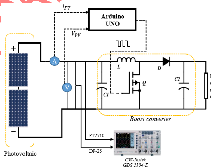
Figure 2. Block diagram of the MPPT system testing
