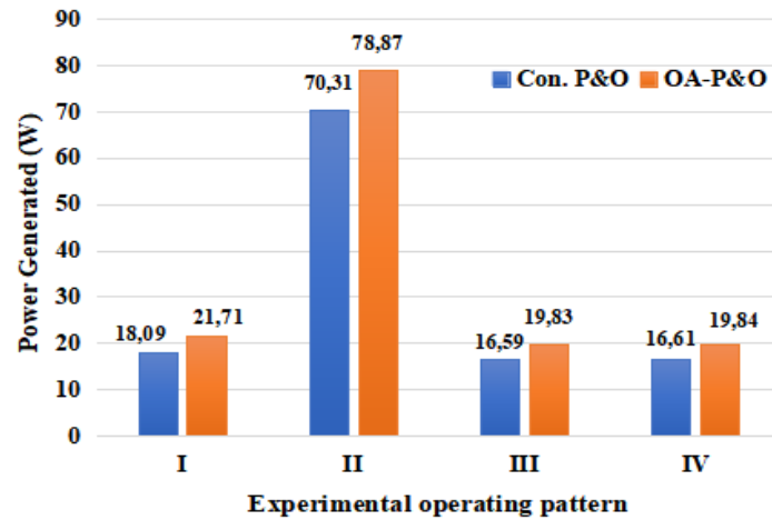
Figure 7. Comparative average power generated under experimental operating pattern
